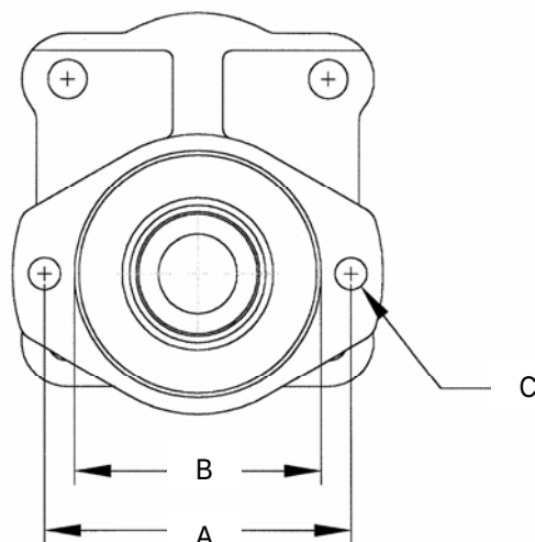
2 Bolt "C" Mount
