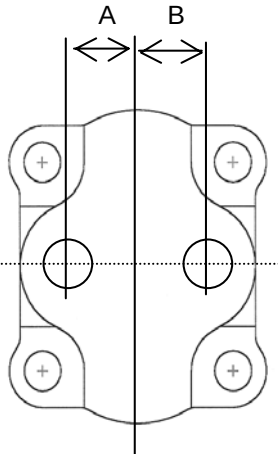
ORIENTATION IS FROM THE SHAFT END
