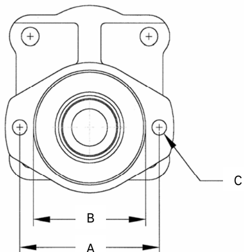
2 Bolt "B" Mount
