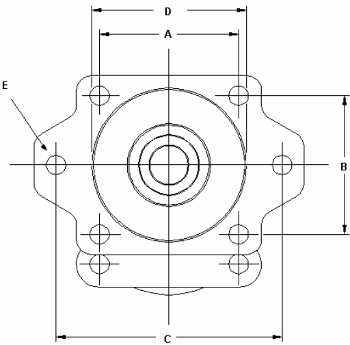
2/4 Bolt C mount
